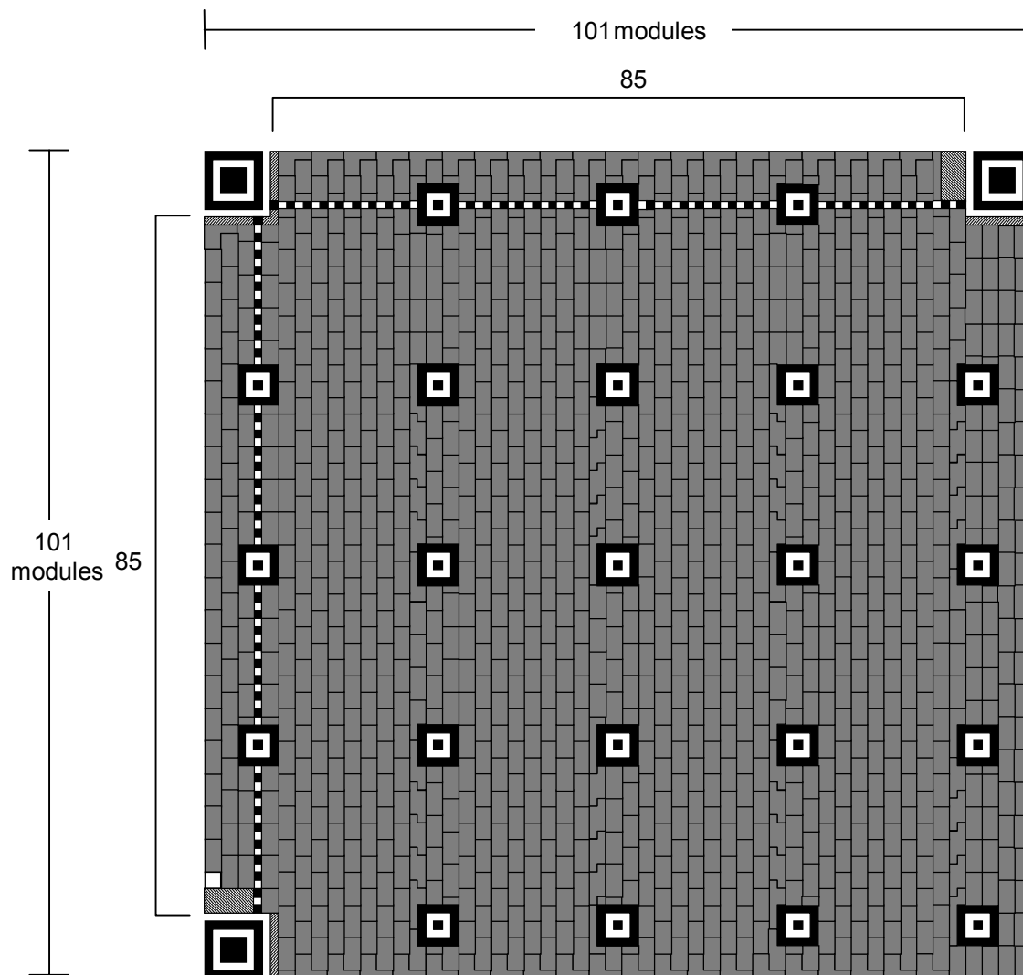
Version 21
