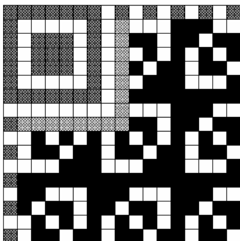
Mask Pattern 10
