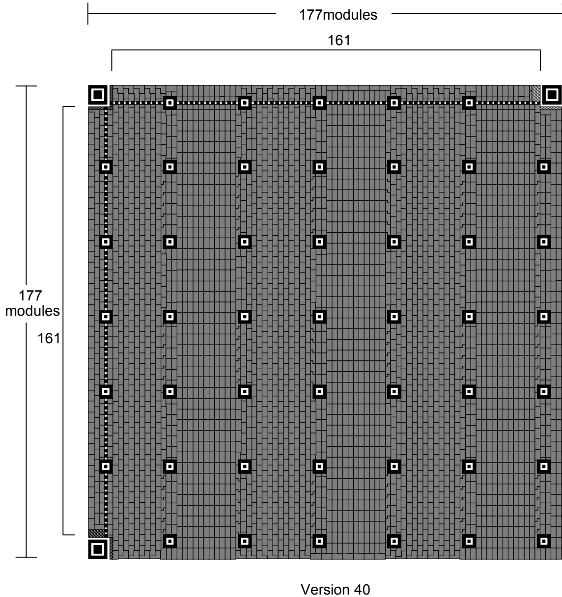
Figure 10 — Version 40 symbol
